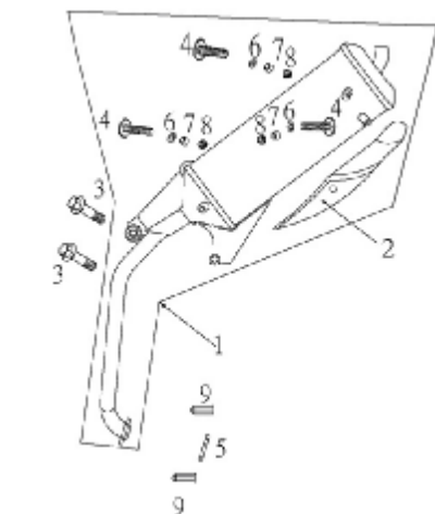
F7 MUFFLER
