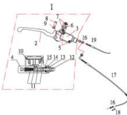
F16 FRONT MASTER CYLINDER
