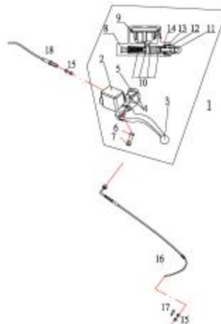
F17 REAR MASTER CYLINDER
