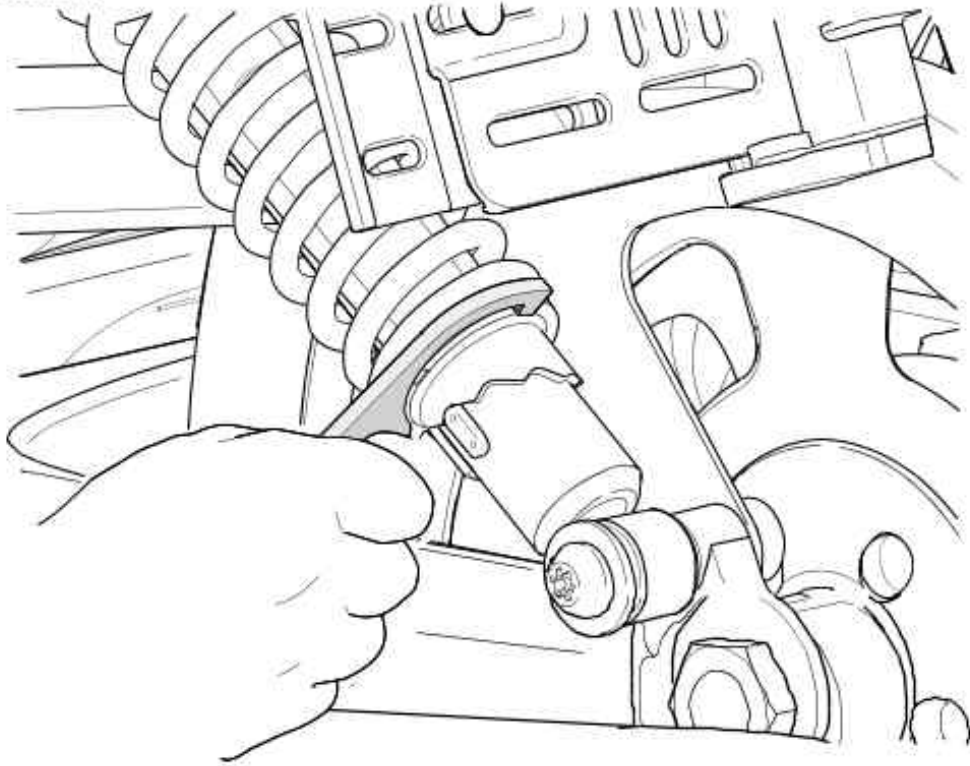
Rear Shock Absorber Adjustment: VRSCF Model
