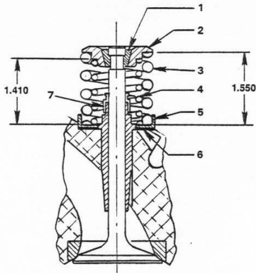
VALVE SPRING SET-UP, INTAKE & EXHAUST 1980 & LATER
