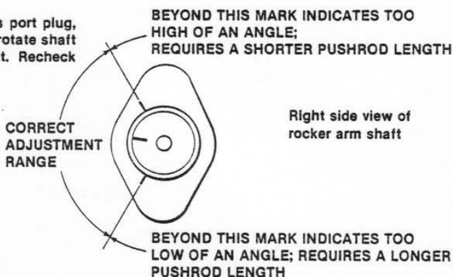
TAPPET ADJUSTMENT
