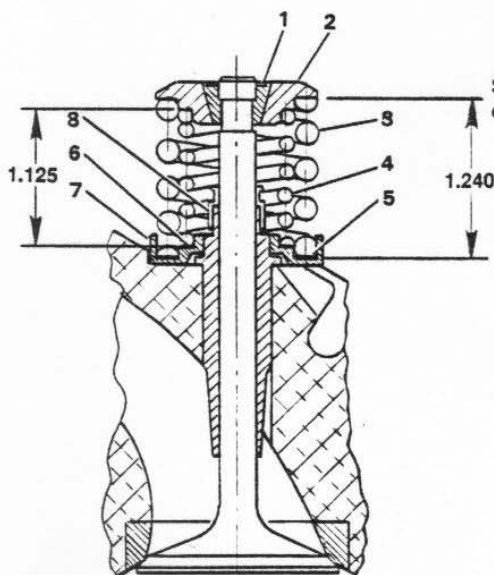
VALVE SPRING SET-UP, INTAKE & EXHAUST 1978 & EARLIER
